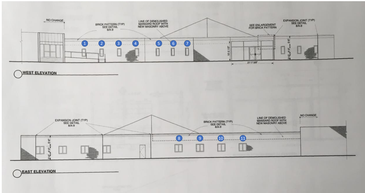
Figure 1 – Township Building, West and East Elevations w/ Window Callouts
